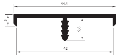
MD 1043 42 S Chipboard
