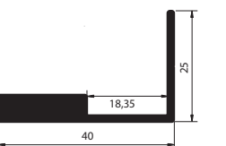
MD 1106 C 18 S Chipboard
