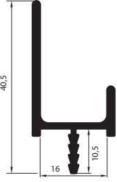
MD 1034 18 19 S Chipboard
