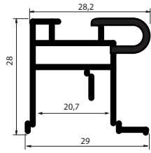
SR 1770 NEW! 8-18 mm Boykulp
