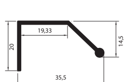
MD 1024 18 S Chipboard
