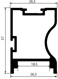
SR 2080 NEW! 8-18 mm Boykulp
