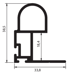
MD 1075 18 mm Suntalam/Chipboard
