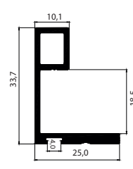
MD 1089 B 18 mm Suntalam/Chipboard
