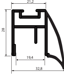
SR 1771 NEW! 8-18 mm Boykulp
