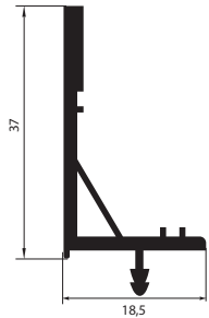
MD 1035 L 18 19 S Chipboard NEW!
