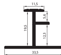
MD 1092 A 18 S Chipboard 4 mm Cam Geçiş / Glass
