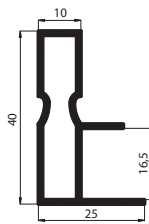
MD 1079 16 mm Suntalam/Chipboard
