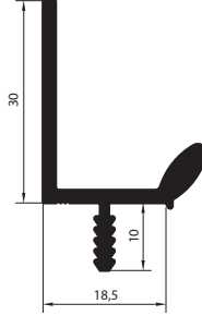
MD 1036 18 19 S Chipboard
