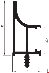
MD 1029 L 18 19 S Chipboard NEW!
